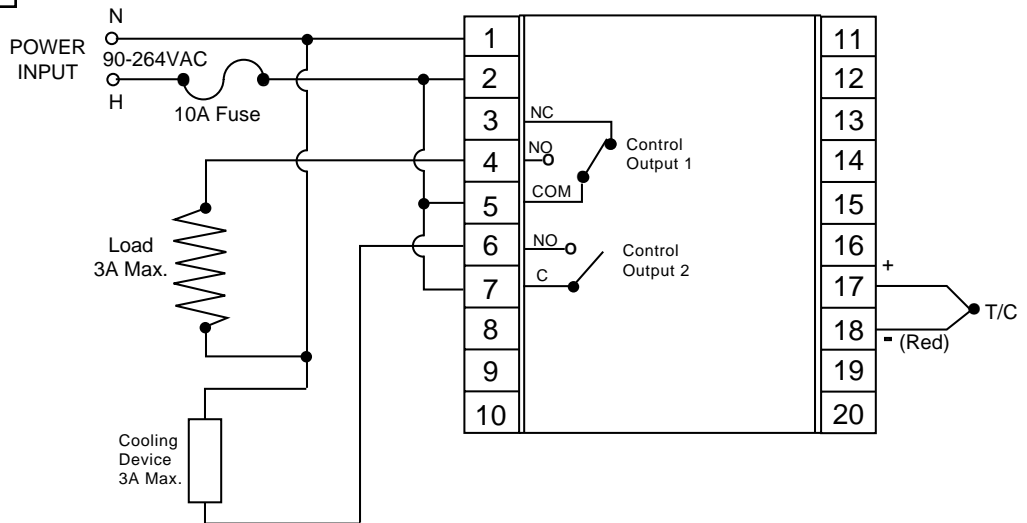
Figure 4.9 ETR-4230-312211 Thermocouple Input. Relay Output for heating and cooling
