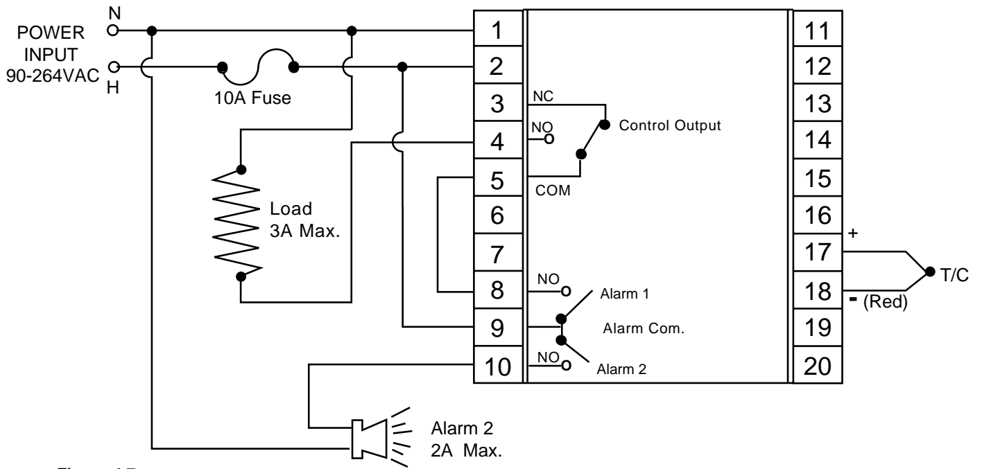
Figure 4.7 ETR-4220-31221 Ramp and Soak Thermocouple Input Relay Output One Alarm Dwell Time Relay Off A1.SF = toof
