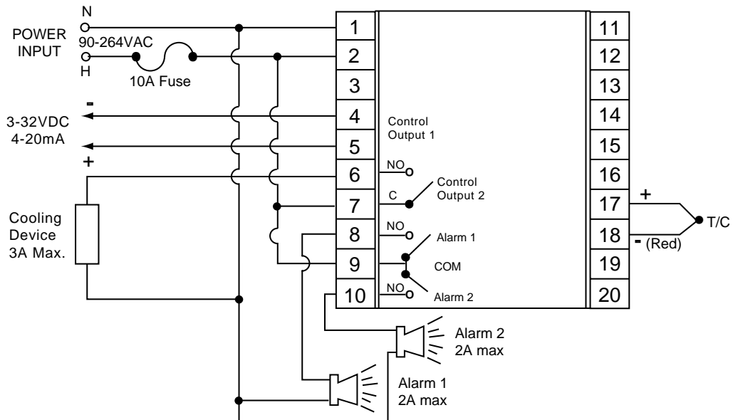
Figure 4.10 ETR-4230-315221 Thermocouple Input 4-20mA Output 1 Relay Output 2 Dual Alarms
