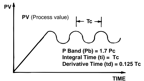
Fig. 5.3 Steady State Cycling
