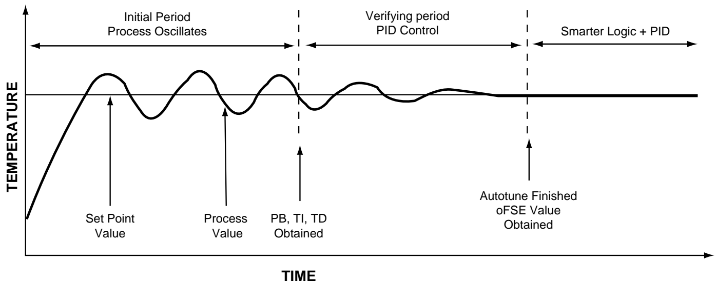
Figure 5.1 Autotuning
